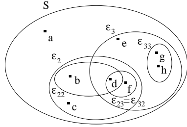
Figure 4. A HyperSet
