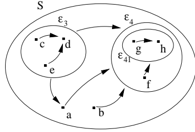
Figure 6. A HyperNodeGraph
