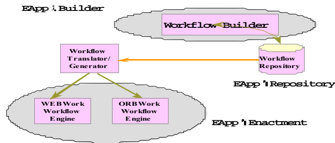
Figure 1: METEOR Architecture
