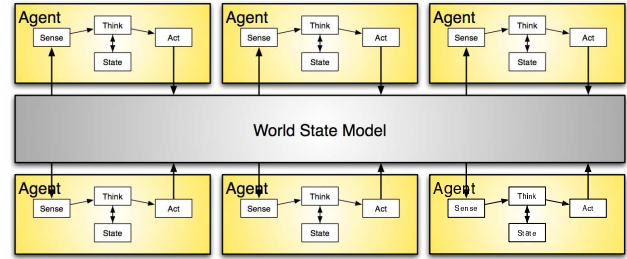
Figure 3: An Agent-Based Simulation
